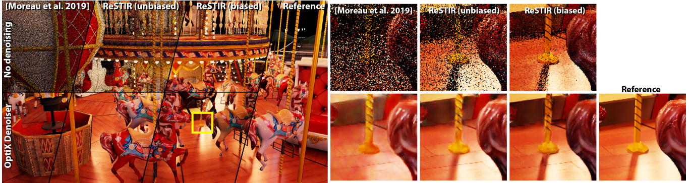
Fig. 2. While existing denoisers (e.g., Chaitanya et al. [2017]; NVIDIA Research [2017]; Schied et al. [2018]) vastly improve image quality at a given sampling rate, they cannot reconstruct features that are missing from their input samples. Our work improves the sampling quality at a given computation budget, enabling existing denoisers to produce better results. Here we show Moreau et al. [2019]’s light BVH, our unbiased (Section 4) and biased (Section 3) methods with and without the OptiX denoiser [NVIDIA Research 2017]. The AMUSEMENT PARK’s carousel image is rendered in 42 ms at 1920 \times 1080 resolution (without denoising) with 3.4 million animated lights. Carousel ©carousel_world
