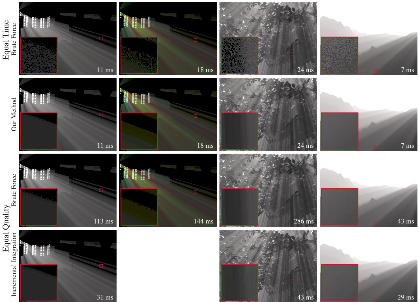
Figure 6: A comparison of our method to brute force ray marching and incremental integration. The GPU implementation of incremental integration does not support colored textured light sources and is therefore omitted. The reported times are for the scattering computation only, excluding the time to render the shadow map, the depth map, and to compute direct lighting.
