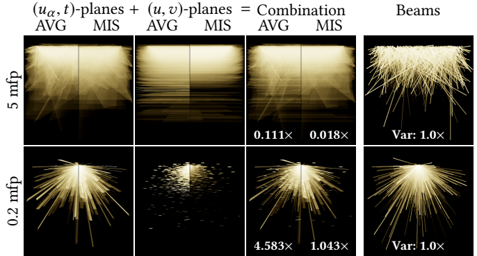
Fig. 6. We examine the effect of light source size (rows) on the relative performance of continuously rotated (u_\alpha, t) -planes (first column) and (u, v) -planes (second column). For each estimator we show its contribution individually (left split, AVG), as well as weighted by MIS (right split). The third column shows the weighted and unweighted combination of these two estimators, as well as their variance (relative to beams). The (u, v) -planes perform well for large light sources, but for smaller lights their weight diminishes compared to (u_\alpha, t) -planes, which start to resemble the photon beams baseline, though without bias. Expanded comparison is in the supplemental.
