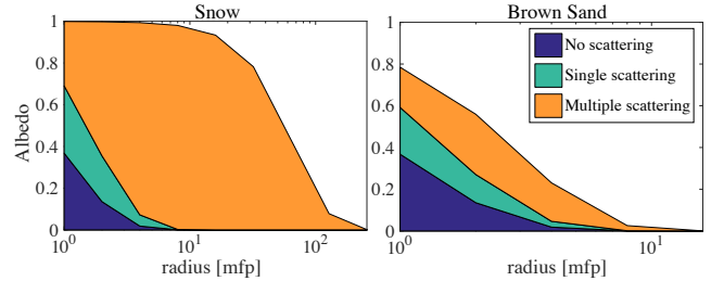
Figure 9: Normalized contributions of individual components (uncollided, single-scattered, and multi-scattered flux) to the total albedo vary with the radius of the shell (measured in mean free paths).
