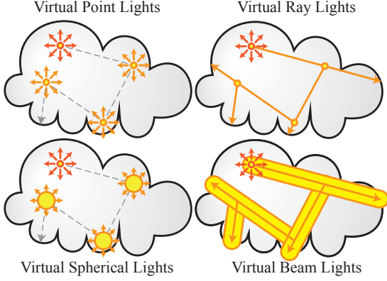
Figure 2: Left: we are inspired by VSLs (bottom), which expand VPLs (top) into spheres with finite solid angle. Right: we similarly expand VRLs (top) into VBLs (bottom) with finite thickness. This removes singularities and reduces render time for indirect lighting to and from surfaces and media.
