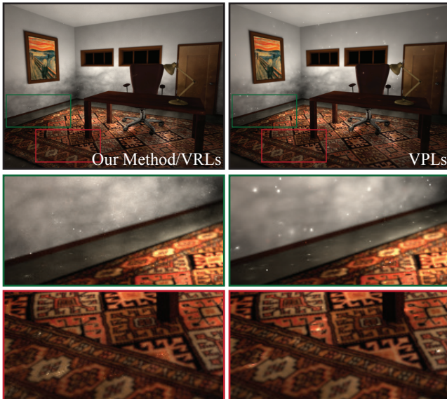
Figure 11: These images show volume-to-surface transport in the SMOKY ROOM scene computed in only 600s; some regions are dark also due to absorption and out-scattering in the participating media. The close-ups compare the singularities of VRLs and VPLs (both without clamping).
