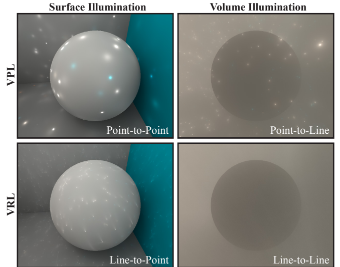
Figure 9: We analyze four different cases of energy transfer; for illustration we use an equal number (10k) of VPLs and VRLs to render a sphere in participating media. The left column shows surface illumination only. Top row: light transport computed using VPLs; bottom row: VRLs illuminating surfaces and media.
