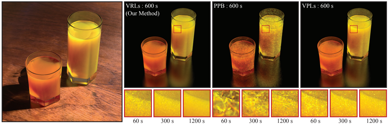
Figure 1: The FRUIT JUICE scene featuring both single and multiple scattering (left). We evaluate the quality of multiple scattering. Our approach can compute the multiple scattering within the media in about a minute (middle-left), while in equal time, both the previous state-of-the-art approaches for general media (progressive photon beams, middle-right; virtual point lights, right) contain significant artifacts.
