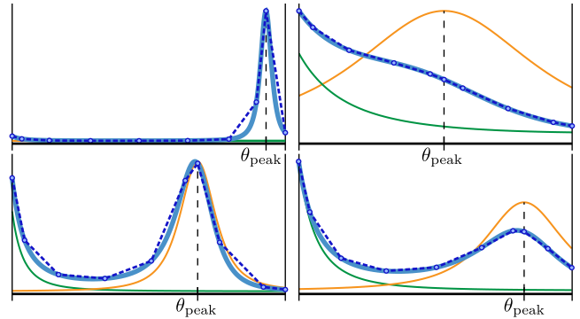
Figure 6: Four example configurations of anisotropic phase functions (Henyey-Greenstein with g = 0.95 ) plotted along the angular domain about a point v_i on the VRL. The product of the phase function along the camera ray (green) and along the VRL (orange) results in the product (solid blue) to which we fit a piecewise-linear PDF (dashed blue). With only 10 vertices, we can reconstruct the product robustly for arbitrary configurations.
