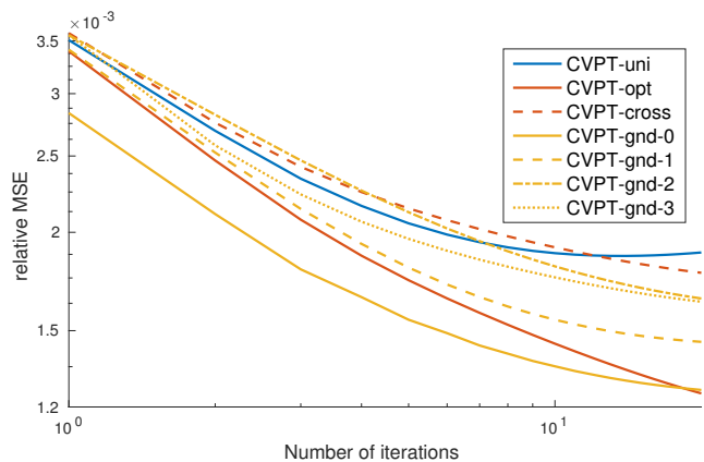
Figure 8: We plot the relative MSE as a function of the number of iterations, when reconstructing the SPONZA scene (rendered with 64 samples per pixel) with our iterated schemes driven by noisy statistics, and weighted reconstructions driven by ground truth statistics, using zero, one, two, or all three of our assumptions (CVPT-gnd-0 to CVPT-gnd-3), illustrating the cumulative impact of our assumptions on the reconstruction quality.
