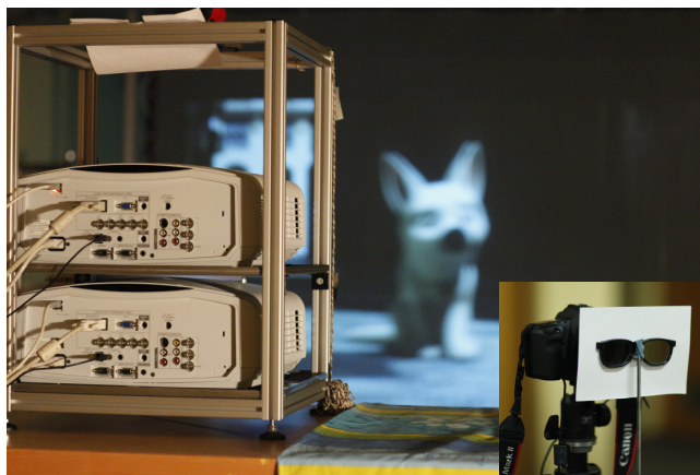
Figure 5: Our experimental rear-projection setup consisting of two projectors using polarization filtering for generating separate left and right eye images. Results are captured by mounting the eyewear in front of a camera lens (inset).
