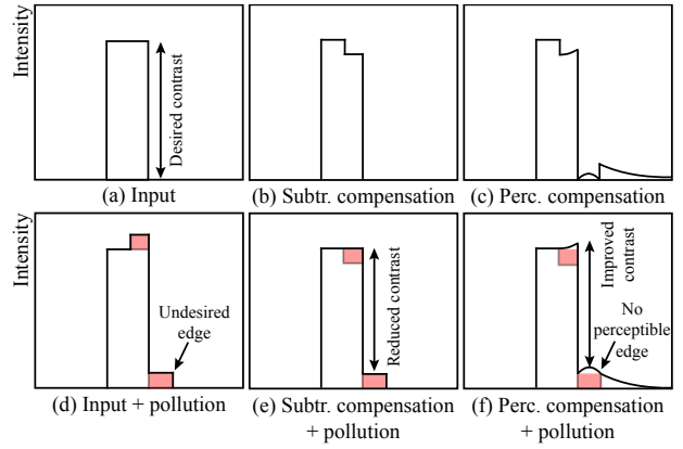
Figure 4: A 1-D illustration comparing no compensation, subtractive compensation and CSF weighting (perceptual) compensation. (a)-(c) The input images. (d)-(f) The observed images. Pollution is depicted as the red shaded areas. Perceptual compensation smoothes the high contrast edge of the ghost, while simultaneously maximizing the contrast of the original input right-hand edge.
