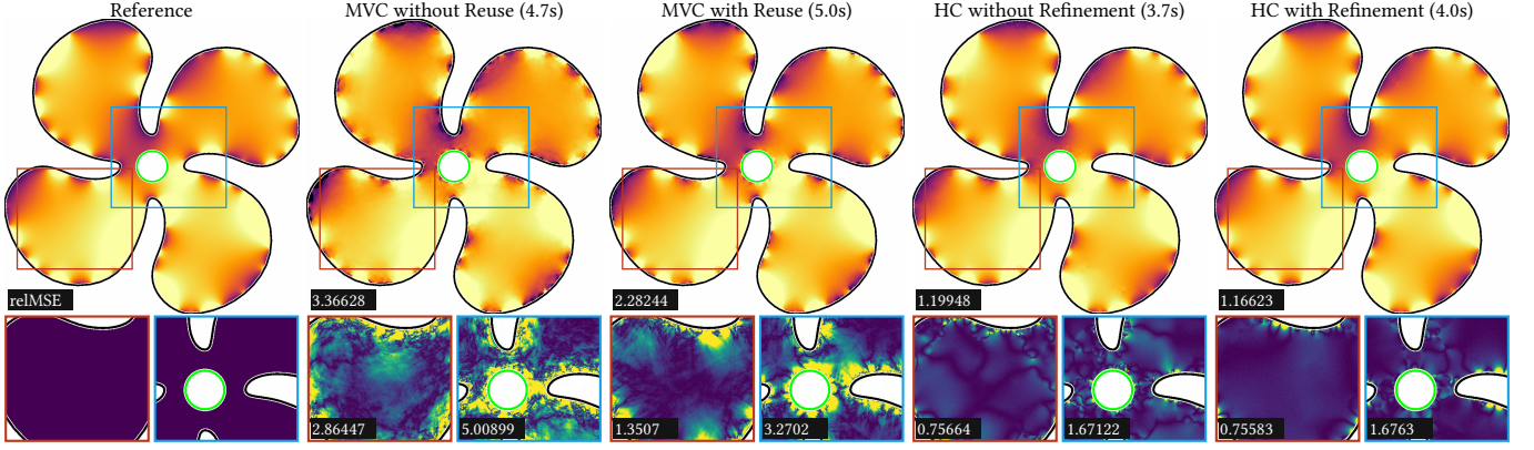
Fig. 13. Reusing the harmonic cache to recompute Fourier coefficients in a refinement pass reduces correlation artifacts and lowers error. This approach resembles the recursive reuse pass in mean value caching but achieves higher accuracy, particularly near boundaries.
