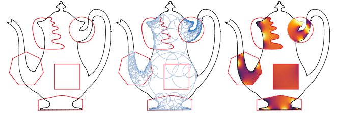
Fig. 4. Overview of our harmonic caching algorithm for solving elliptic PDEs. We leverage the generalized mean value property of harmonic functions (Fig. 2) to reconstruct solutions from local boundary estimates. Within user-specified regions of interest (left), we adaptively place overlapping spherical cache records (middle), each storing a compact set of Fourier coefficients. Blending local reconstructions from each record yields a smooth, low-error approximation across the region (right).
