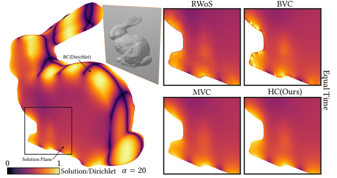
Fig. 8. Harmonic caching shows fewer correlation artifacts in the interior than RwS (top-left inset) and less noise near the boundary than MVC (bottom-left inset). Unlike BVC (top-right inset), it also free of singularity issues near the boundary. Results shown for a screened 3D Laplace problem.
