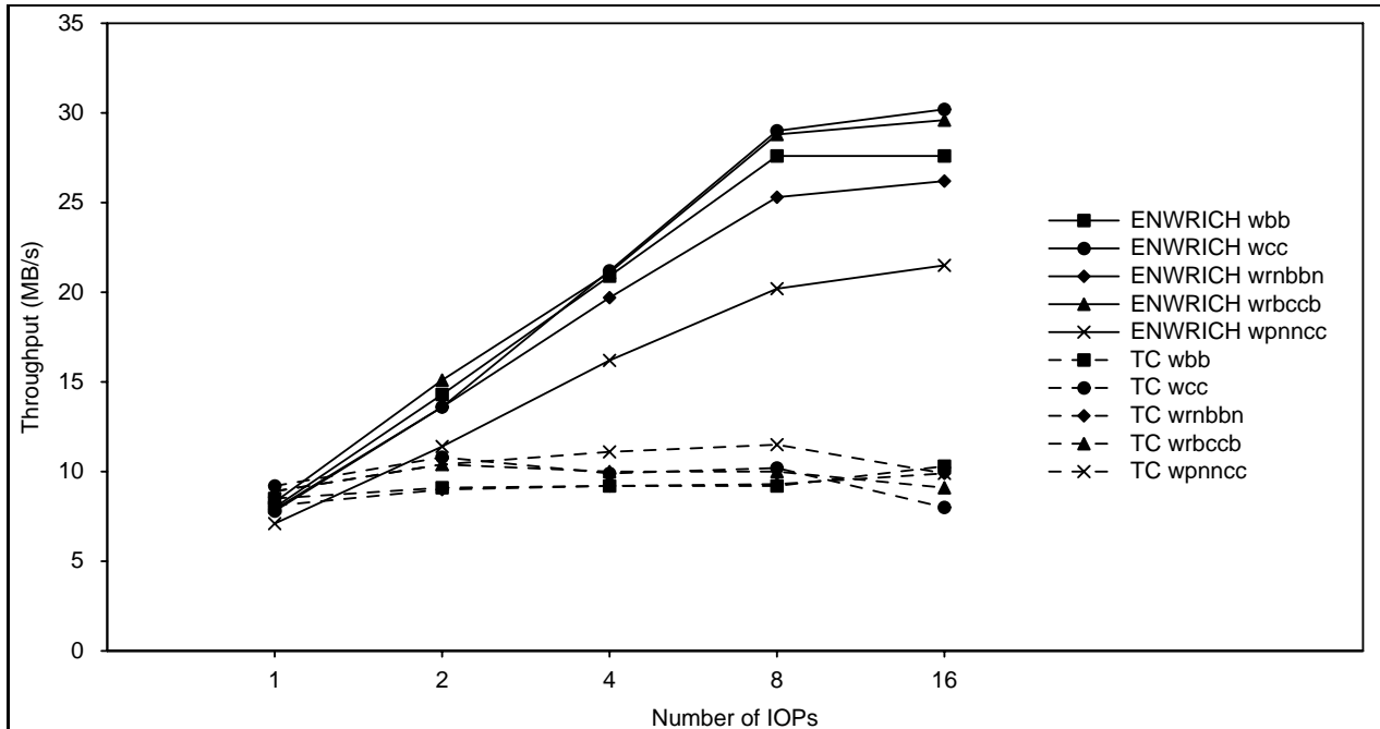
Figure 8: Graph showing performance variations of ENWRICH and TC with changing number of IOPs for some patterns. The number of CPs and disks were kept at 16. All experiments used a contiguous disk layout, 8192-byte records, and 64 MB files. Per-CP cache size for ENWRICH experiments was fixed at 1 MB.
