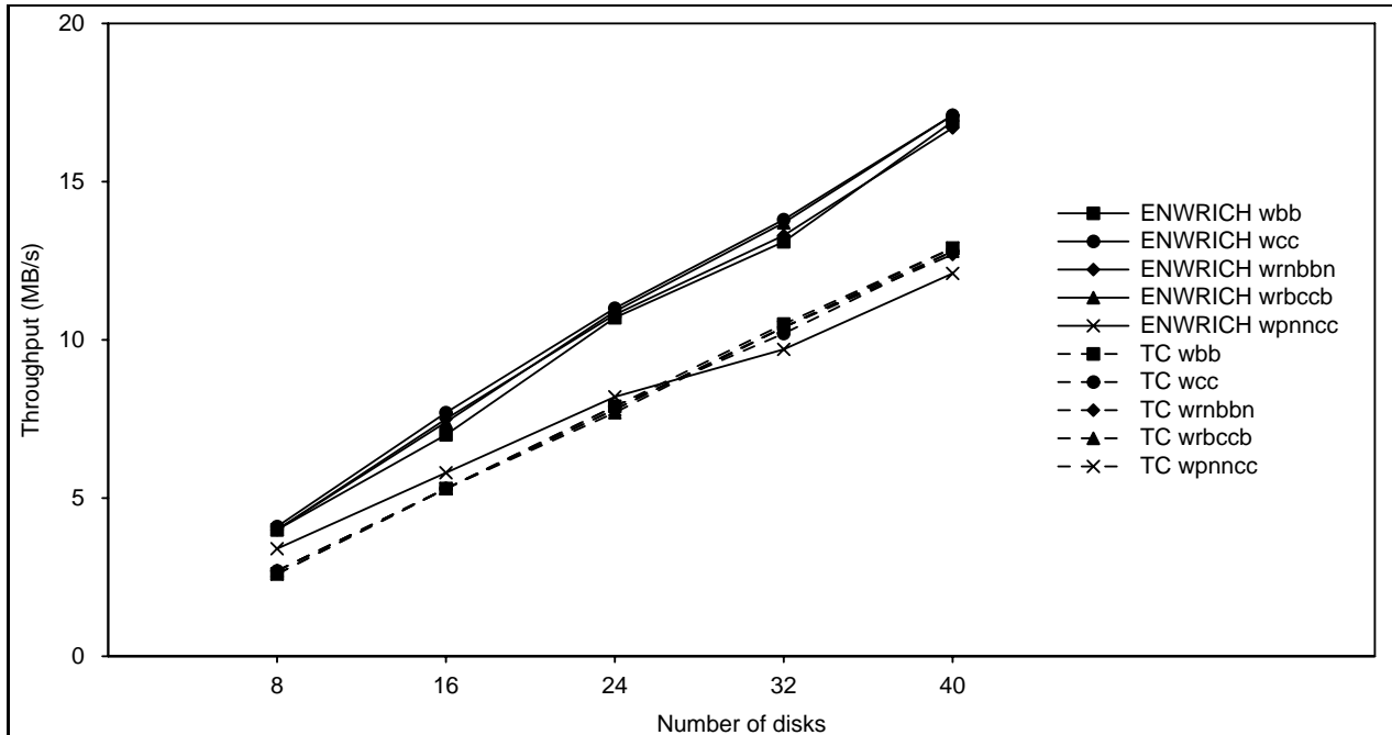
Figure 10: Graph showing performance variations of ENWRICH and TC for some patterns, varying the number of disks and using a random-blocks layout. There were 16 CPs and 8 IOPs in all the experiments. The ENWRICH cache size was fixed at 1 MB per CP.
