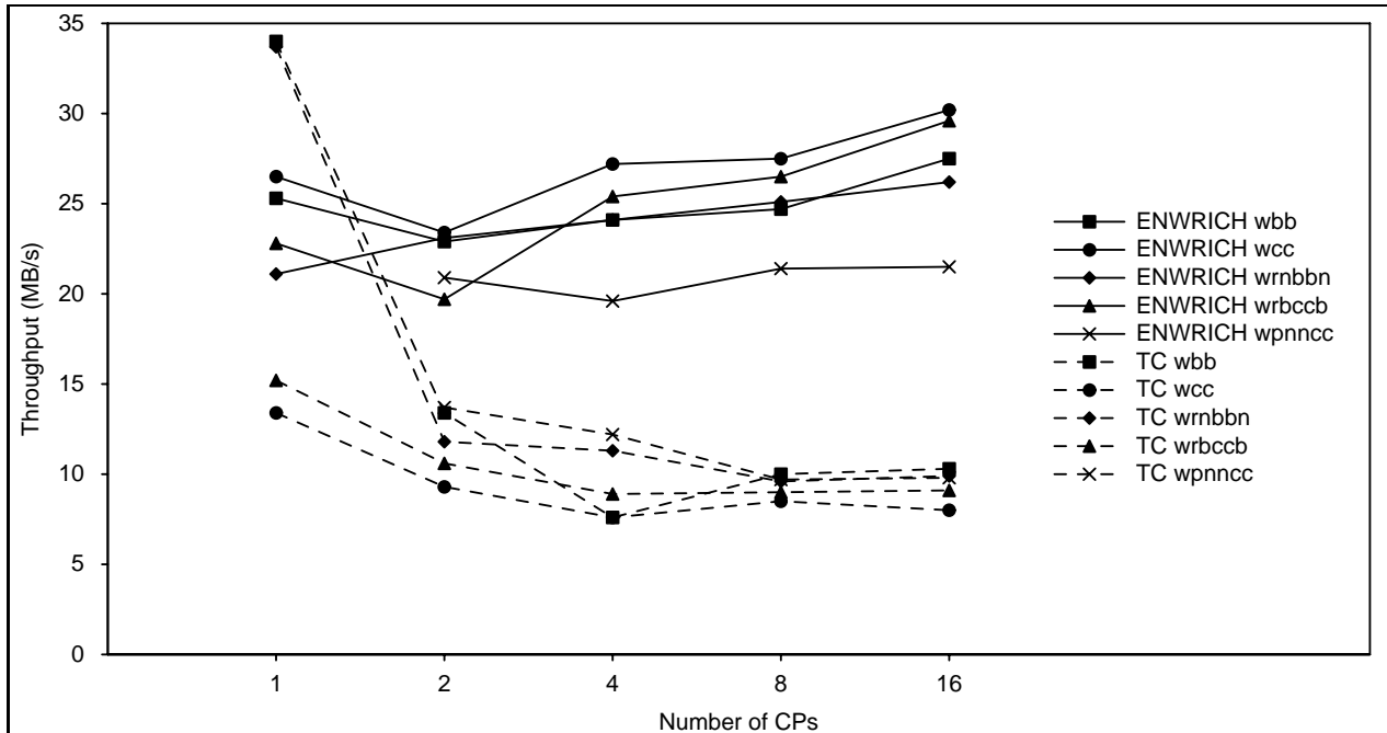
Figure 7: Graph showing performance variations of ENWRICH and TC with a changing number of CPUs for some patterns. The number of IOPs and disks were kept at 16. All experiments used contiguous disk layout, 8192-byte records, and 64 MB files. Per-CP cache size for ENWRICH experiments was fixed at 1 MB.
