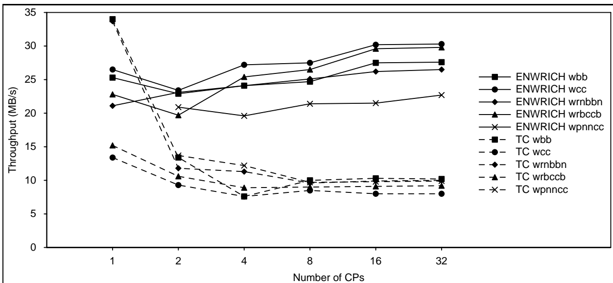
Figure 7: Graph showing performance variations of ENWRICH and TC with a changing number of CPUs for some patterns. The number of IOPs and disks were kept at 16. All experiments used contiguous disk layout, 8192-byte records, and 64 MB files. Per-CP cache size for ENWRICH experiments was fixed at 1 MB.
