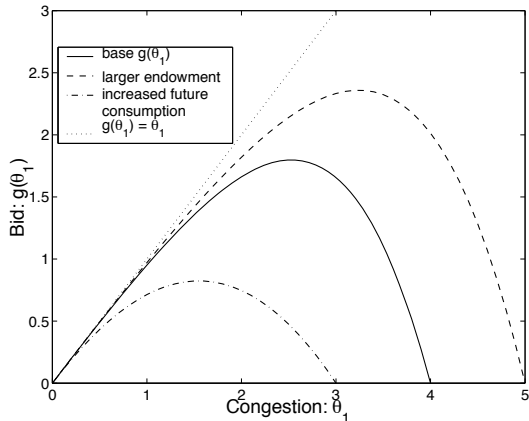
Fig. 0.4. The form of an agent’s bid as a function of all bids submitted to the server. As the agent’s endowment increases, the function scales outward. Increasing the size of future tasks results in a smaller gentler curve.
