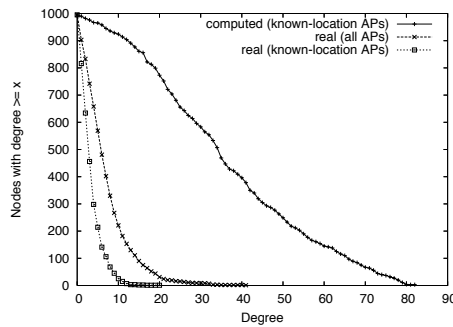
Fig. 12. AP degrees. ‘computed’ denotes degrees computed with the 50 m interference assumption. Two ‘real’ lines present degrees observed by APs: one with all APs and the other including only the APs with known locations.
