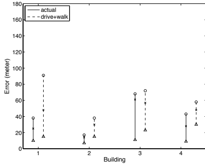
Fig. 8. Error in indoor user location, computed every 10 seconds. ( \triangle :50%, \times :95%, \circ :100%).
