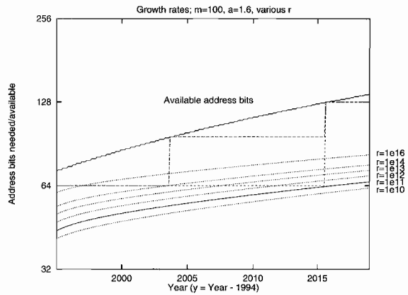
Figure 6. Comparison of available address bits with the consumption of address space for a variety of current rates, r , but with an acceleration factor of a = 1.6 , and m = 100 . The solid consumption curve indicates the r value used in the other graphs.
