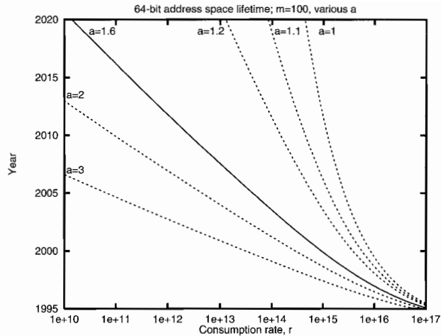
Figure 9. Comparison of various acceleration factors ( a ), showing the year in which a 64-bit address space will be completely consumed based on the initial rate ( r ). The solid curve indicates the a value used in the other graphs. We assume a 1994 start, and add m = 100 machines per year.
