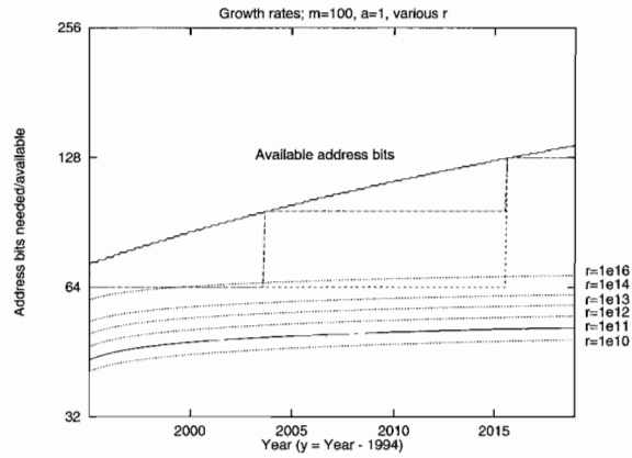
Figure 5. Comparison of available address bits with the consumption of address space for a variety of current rates, r , assuming no acceleration ( a = 1 ) and m = 100 . The solid consumption curve indicates the r value used in the other graphs. The available address bits grow in increments of 1, 32, or 64 bits.
