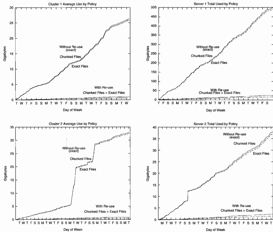
Figure 3. Cumulative address space consumed under different management policies, for each tracing group, over the interval traced. Curves for Cluster 1 and Cluster 2 are scaled down by the number of machines in each cluster, for easier comparison. x -axis tic-marks represent midnight before the given day of the week. The “fixed” file and process policies were so much worse that they are not shown (see Table 3).
