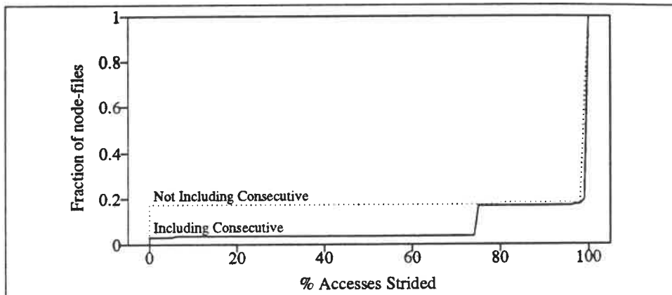
Figure 1: Cumulative distribution of node-files according to the fraction of accesses that were involved in a simple-strided pattern. This graph covers both the case where consecutive accesses are counted as strided (with an interval of 0) and the case where they are not.
