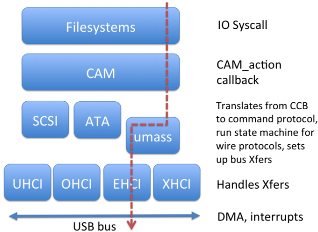
Figure 4: Path of a bus IO request through USB stack layers.
