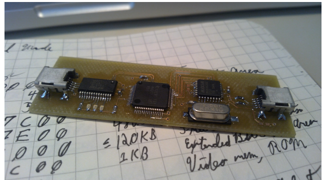
Figure 6: Facedancer, a USB device emulator.
