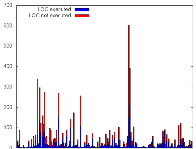
Figure 5: For each function, the number of lines of code executed while processing an ordinary I/O request (blue) overlaid on the total number of lines of code (red). Each point on the x-axis represents a distinct function within FreeBSD’s USB stack.
