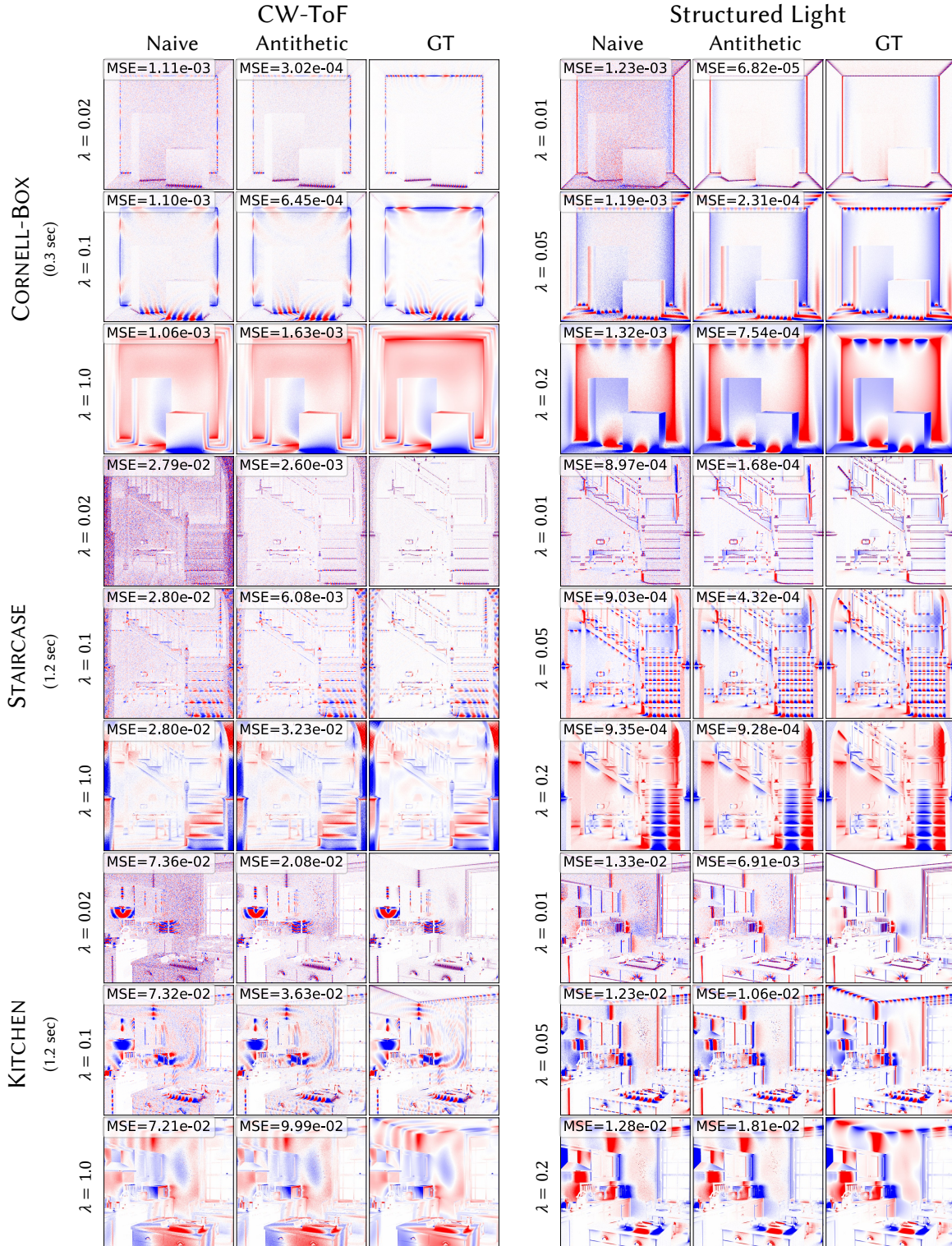
Fig. 10. Equal-time comparison of modulated indirect illumination rendered using naive and antithetic sampling across multiple scenes and wavelengths. Per-image MSE values are reported above each result. Antithetic sampling substantially reduces noise at short wavelengths, while its advantage decreases at longer wavelengths as the required geometric deformation increases. Complete MSE curves are shown in Fig. 4.
