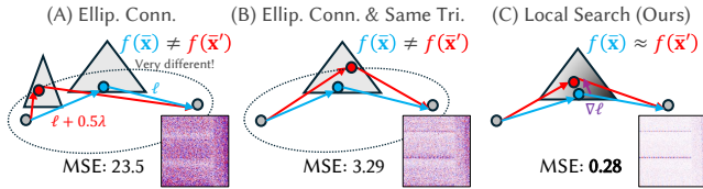
Fig. 7. Comparison of antithetic path construction strategies on STAIRCASE. (A) Ellipsoidal connection satisfies the path-length constraint but lacks path similarity. (B) Restricting it to the same triangle improves similarity. (C) Our local search best preserves path similarity and achieves the lowest MSE.
