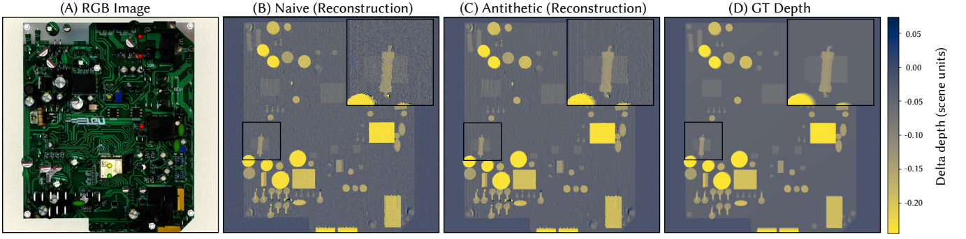
Fig. 11. Fringe projection profilometry for automated optical inspection. (A) Rendered RGB image of a circuit board. (B–C) Depth reconstructions obtained using naive and antithetic sampling. (D) Ground-truth depth. Depth is recovered from four phase-shifted sinusoidal patterns through phase decoding, spatial unwrapping, and projector–camera triangulation. All depth images use the same colormap and range. Antithetic sampling reduces indirect-illumination noise, improving phase stability and reconstruction accuracy. Residual deviations from ground truth arise from global illumination and texture-edge artifacts, which also occur in real-world measurements [Deng et al. 2020; Hu et al. 2023; Shi et al. 2024].
