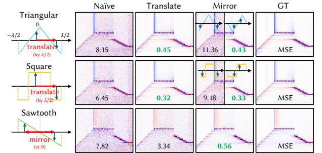
Fig. 6. Comparison of antithetic mappings for triangular, square, and sawtooth patterns. Translation pairs (\xi, \xi + \lambda/2) , while mirroring pairs (\xi, \lambda - \xi) modulo \lambda . Translation is valid for triangular and square waves, whereas mirroring is required for the sawtooth and also becomes valid for the others after a \lambda/4 phase shift.
