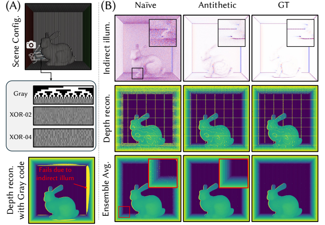
Fig. 8. (A) Depth reconstruction using structured light. Conventional Gray-code decoding often fails in the presence of indirect illumination. The high-frequency-only XOR patterns proposed by Gupta et al. [2011] can be used instead. (B) We render the XOR-02 measurements using naive and antithetic sampling and then perform depth reconstruction. Following Gupta et al. [2011], we also perform ensemble averaging over two XOR patterns to improve the reconstruction.
