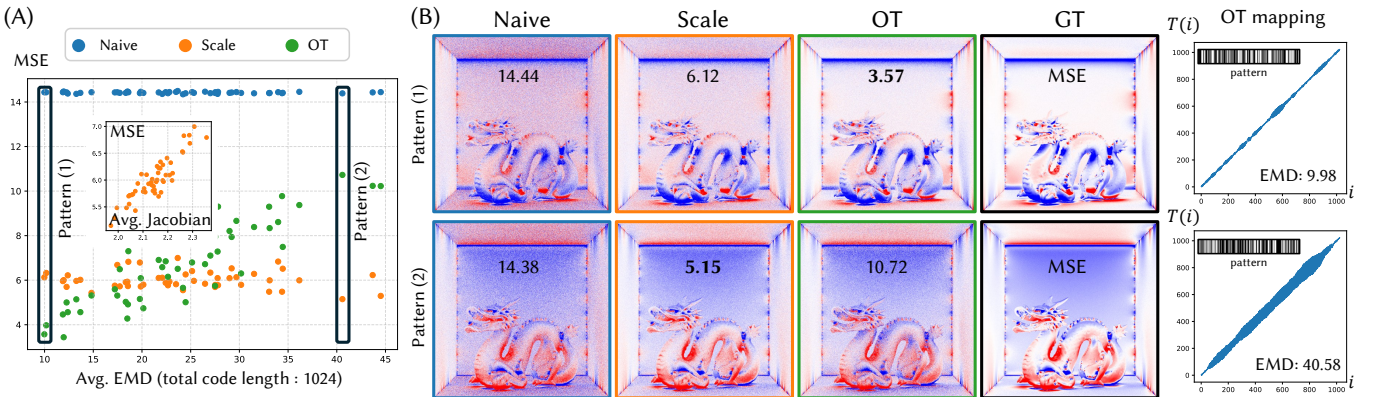
Fig. 13. Comparison of antithetic mappings for 50 arbitrary binary patterns of length 1024. (A) Rendering MSE versus Earth Mover’s Distance (EMD) for naive sampling and antithetic sampling with scale-based and optimal-transport (OT) mappings. OT performs best for low-EMD patterns, while scale-based mapping becomes preferable for patterns with higher EMD; its performance depends instead on the mapping Jacobian. (B) Rendered results and corresponding OT mappings for representative low- and high-EMD patterns, illustrating how larger transport distances reduce path similarity and increase rendering error.
