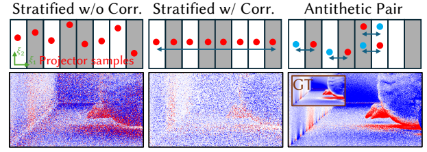
Fig. 9. Comparison with stratified sampling for arbitrary structured-light codes. Uncorrelated samples lack geometric similarity, while sharing \xi_2 reduces path diversity. Our antithetic mapping enables effective cancellation while preserving path diversity.
