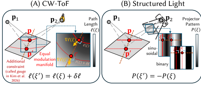
Fig. 2. Geometric construction of antithetic sample pairs for two imaging modalities. (A) For CW-ToF, the antithetic manifold consists of paths whose lengths differ by half a wavelength ( \delta\ell = \pm\lambda/2 ). An average-gradient constraint selects a geometrically similar antithetic path while maintaining bijectivity. (B) For structured light, the antithetic manifold is determined directly by projector coordinates with opposite pattern values.
