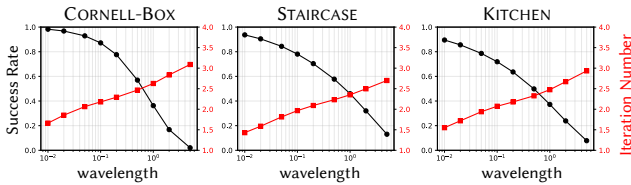
Fig. 5. Newton solver success rate and average iteration count for CW-ToF in Fig. 4. The black line shows the success rate, while the red line shows the average number of iterations. Longer wavelengths require larger path deformations, resulting in lower success rates and more iterations. Successful mappings generally converge within two to three iterations.
