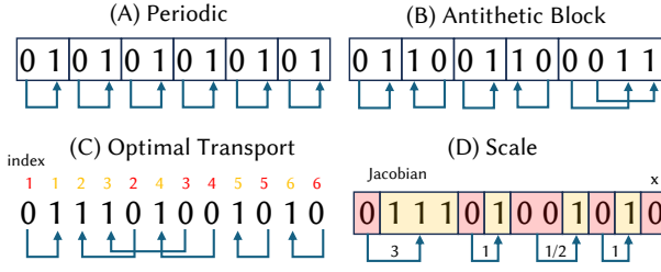
Fig. 3. Antithetic mappings for binary structured-light codes. (A) Periodic codes and (B) aperiodic codes with antithetic blocks admit direct pairing. For arbitrary codes without such blocks, we use (C) optimal transport, with indices of 0s and 1s indicated, or (D) scale-based mapping between contiguous blocks, with the corresponding nonuniform Jacobians shown.
