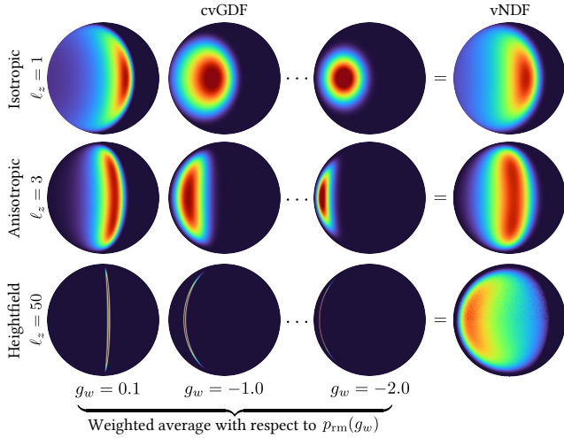
Figure 3: The cvGDF's projections onto the upper hemisphere conditioned on a fixed ray direction \omega_o and different g_w values (left 3 columns). The classical vNDF (right column) corresponds to the weighted average across all g_w \sim p_{rm} generated by ray marching. In the heightfield limit, the vNDF of GPIS (upper half) matches the Beckmann vNDF with Smith approximation (lower half).
